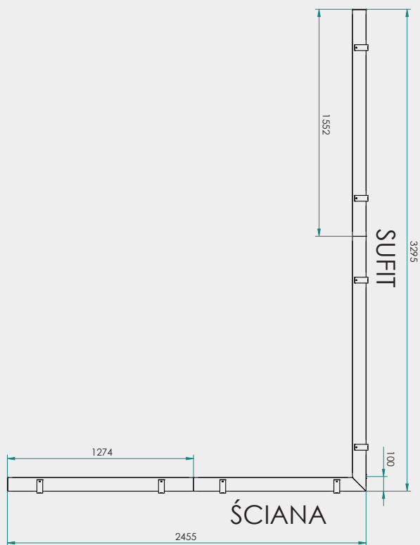
TRU LED 329,5+245,5 recessed, rys. pogl.
